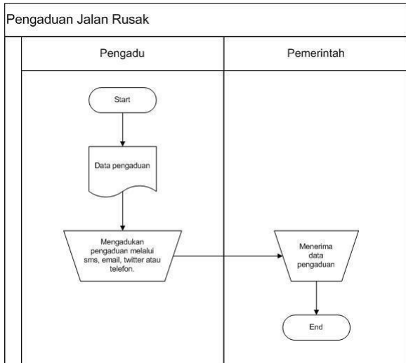
Gambar 3-1 Flowchart Sistem
