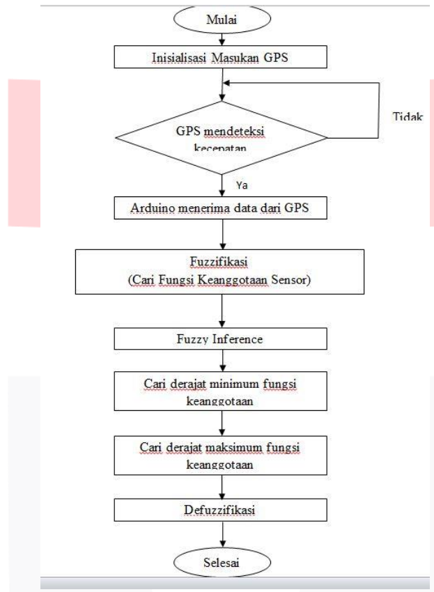
Gambar 3.7 Flowchat Fuzzy Logic
