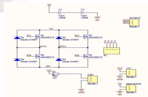
Gambar 3.3b Full Bridge Inverter
