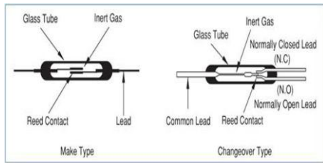
Gambar 2.6 Reed switch [6]
