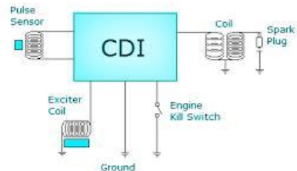
Gambar 2.5 sistem pengapian [8]
