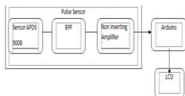
Gambar 7 Blok diagram
