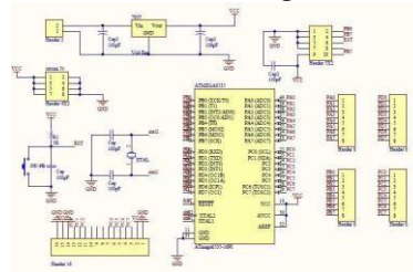
Gambar 3. 3 Sistem Minimum ATmega 8538
