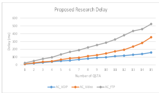
Fig 6. Delay Performance per AC
