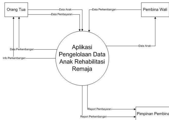
Gambar 2 DFD level 0
