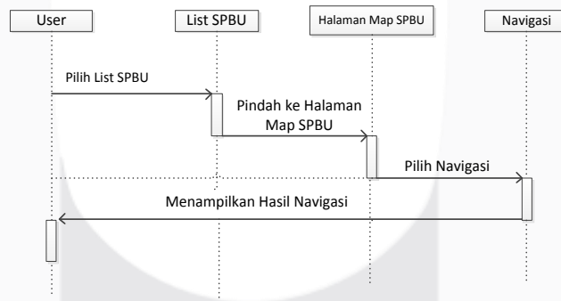
Gambar 4.7 Sequence Diagram Navigasi
