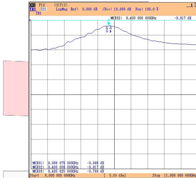
Gambar 4.2 Hasil pengukuran Insertion loss (S21)
