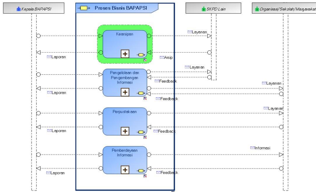
Gambar 3. Business Architecture
