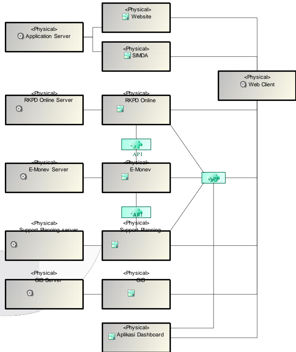
Gambar 6 Platform Decomposition Diagram Target
