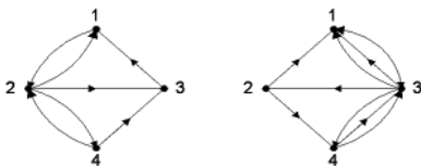
Gambar 2.3 Graph berarah
