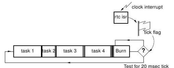
Gambar 2.3 Kehadiran clock tick [6]
