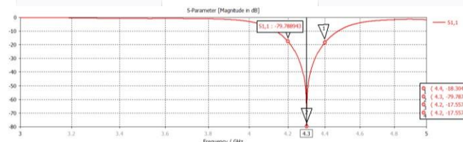
Gambar 3. 3 Return loss 4 Elemen Proximity coupled teknik matching impedance
