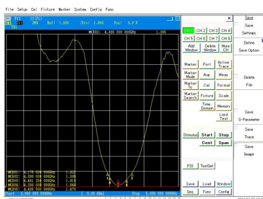
Gambar 4. 1 (a) Hasil pengukuran VSWR di Network Analyzer
