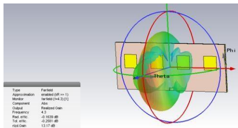
Gambar 3.5 (a) Gain 4 Elemen
