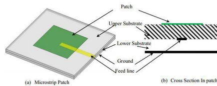
Gambar 2.3 Proximity Coupling [2]
