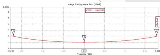
Gambar 3. 4 (a) VSWR 4 Elemen
