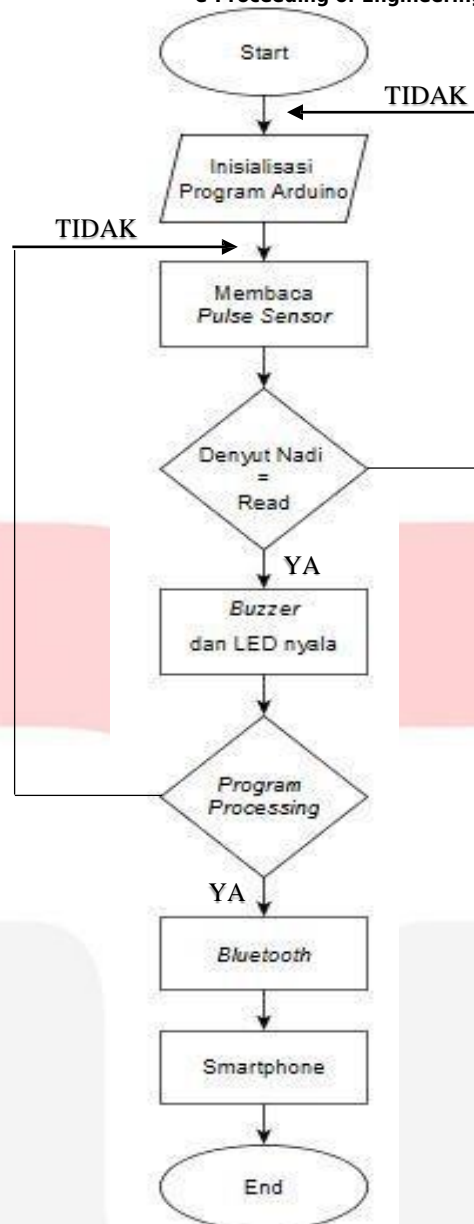
Gambar 3.3 Flowchart Sistem
