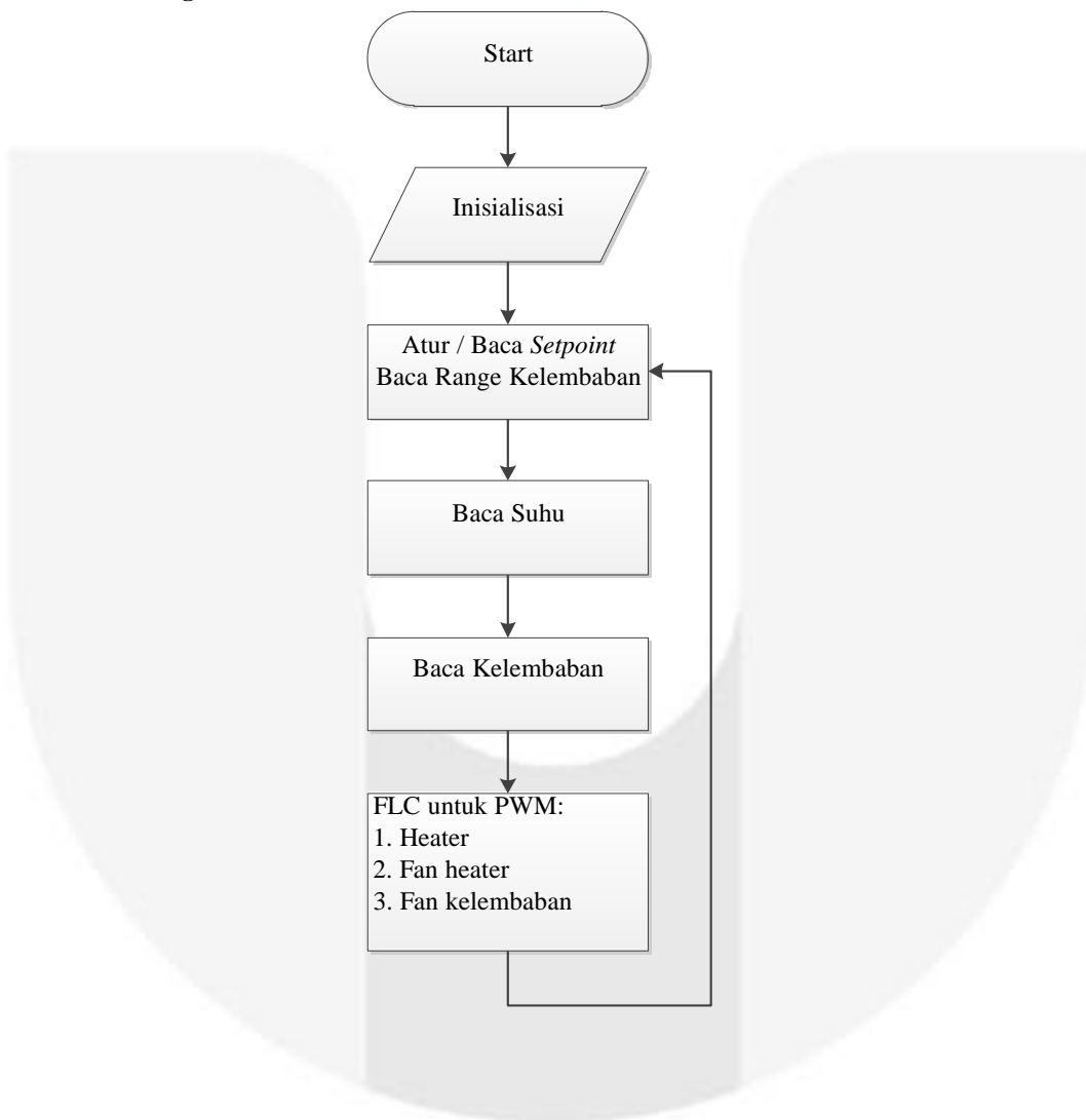
Gambar 2.1. Flowchart Program
