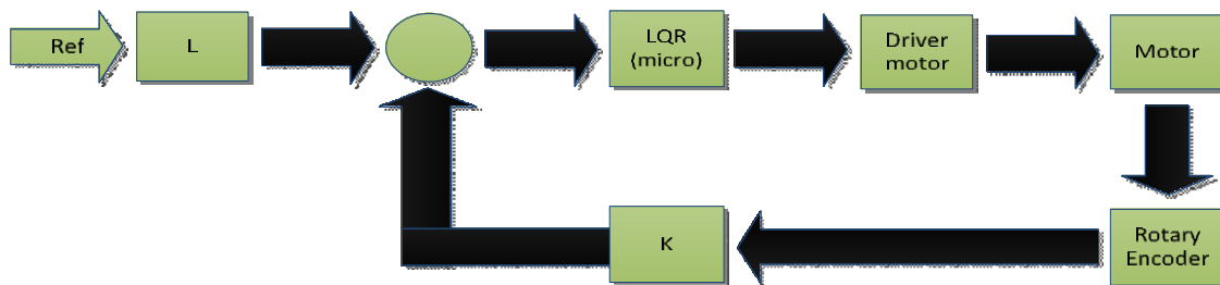
Gambar 3.1 Block Diagram Sistem
