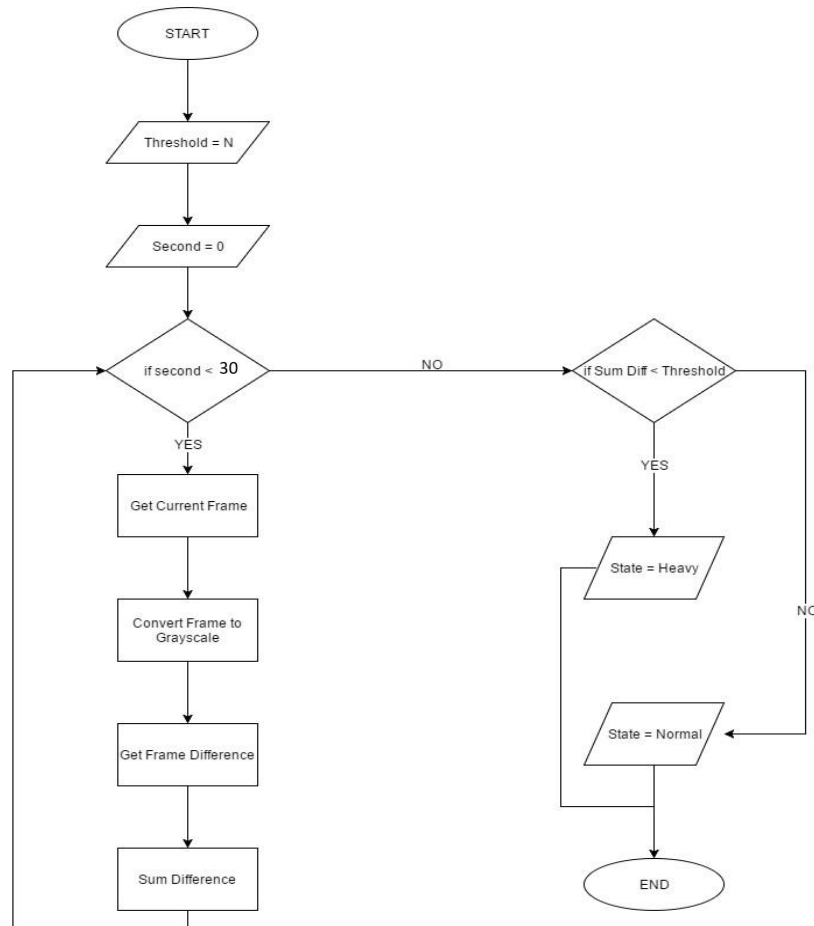
Gambar 3 .4 Blok Diagram Frame Difference dan Penentuan State
