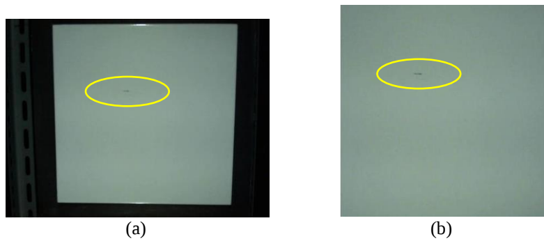
Figure 4 Original defect ceramic (a) and crop ceramic (b)
