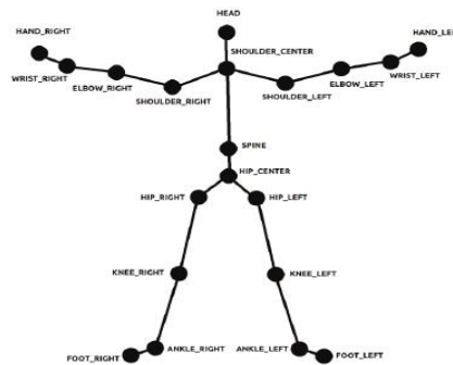
Gambar 1 Skeleton user [6]
