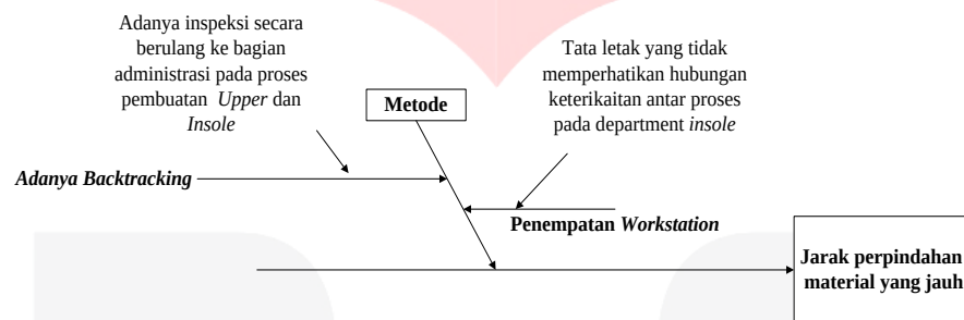
Gambar 4 Fishbone Diagram
