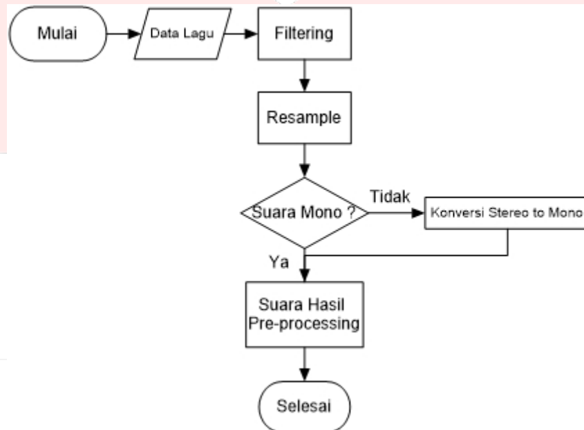
Gambar 3.3 Flowchart Pre-Processing
