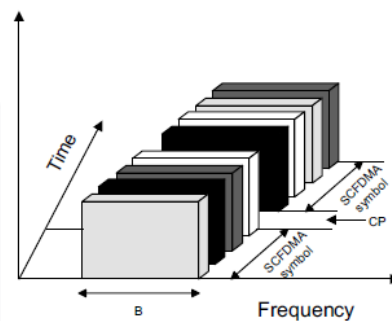
Gambar 2. 1 SC-FDMA [13]
