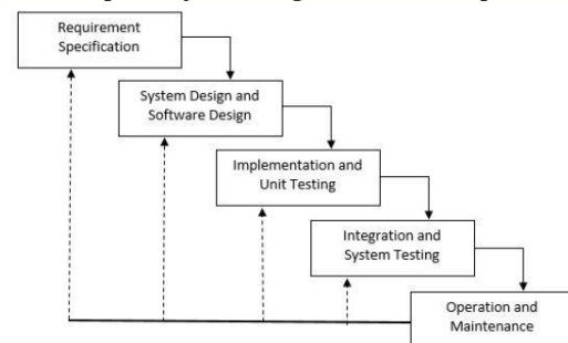
Gambar 1. 1 Model Waterfall [2]
