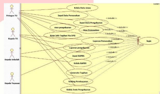
Gambar 3-3 Use Case
