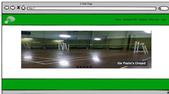
Gambar 3- 24 Tampilan Home
