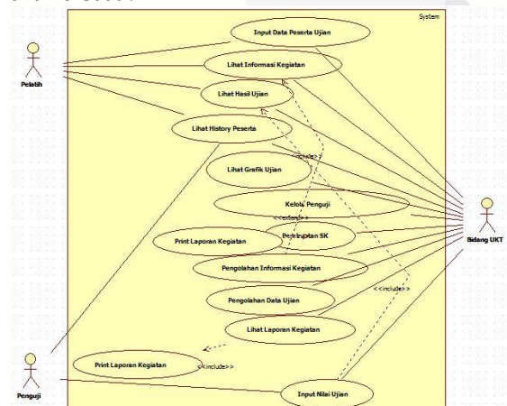
Gambar 3. 7 Usecase Diagram
