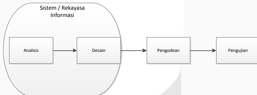
Gambar 1 Model Waterfall
