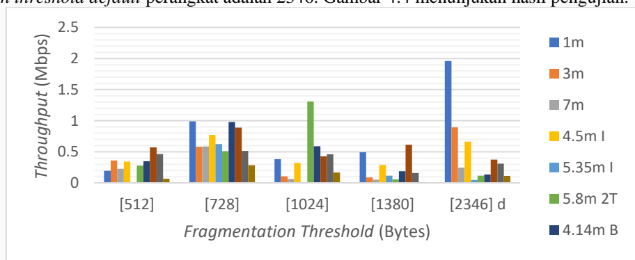
Gambar 3.4 Grafik perubahan nilai fragmentation threshold terhadap throughput
