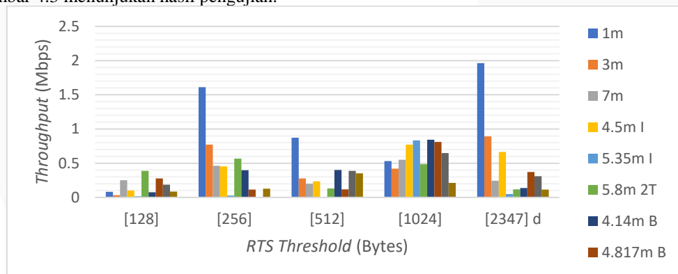
Gambar 3.3 Grafik perubahan nilai RTS threshold terhadap throughput
