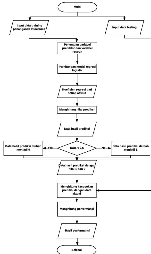
Gambar 3 logistic regression
