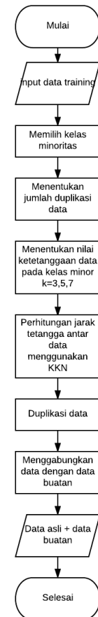
gambar 2 SMOTE
