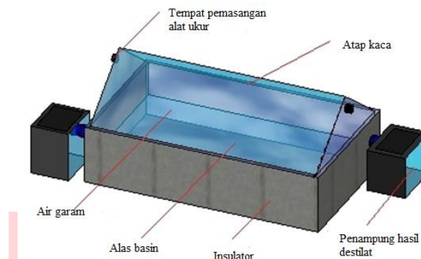
Gambar 2.1 Destilator Surya
