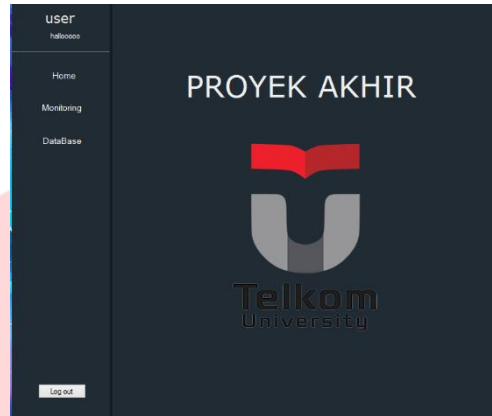
Gambar 4 .3 Tampilan Home
