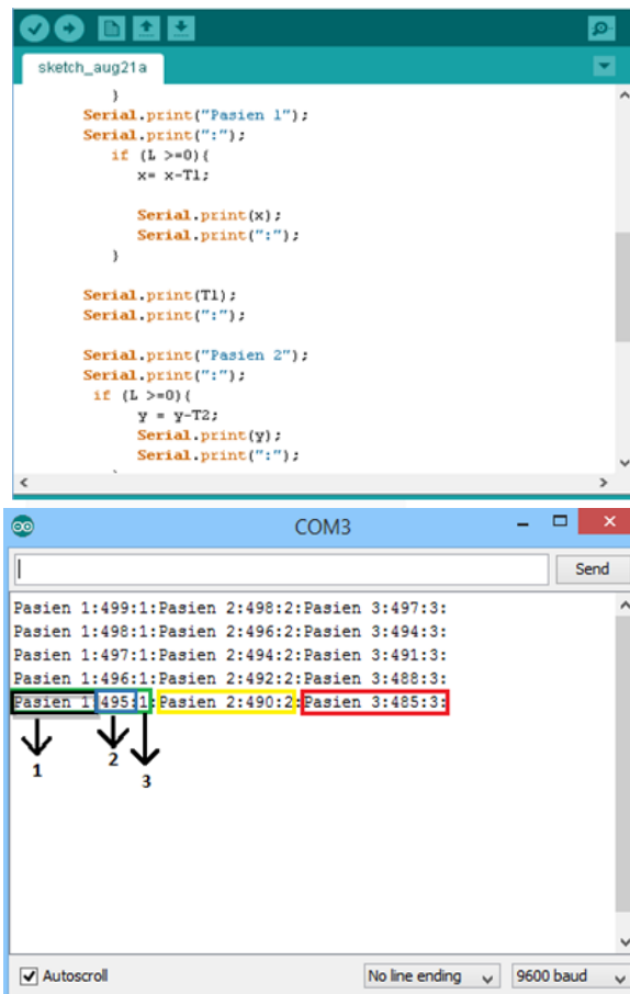
Gambar 3.4 Data Dummy
