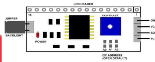
Gambar 2. 7 Modul I2C [10]
