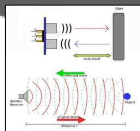
Gambar 2. 1 Cara kerja sensor ultrasonik [3]
