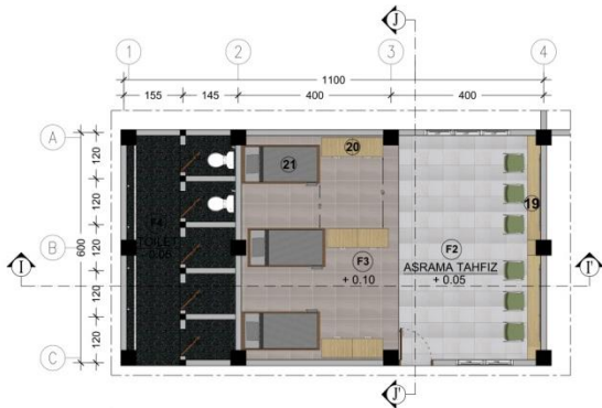
Gambar 6. Layout Kamar Asrama Tahfidz
