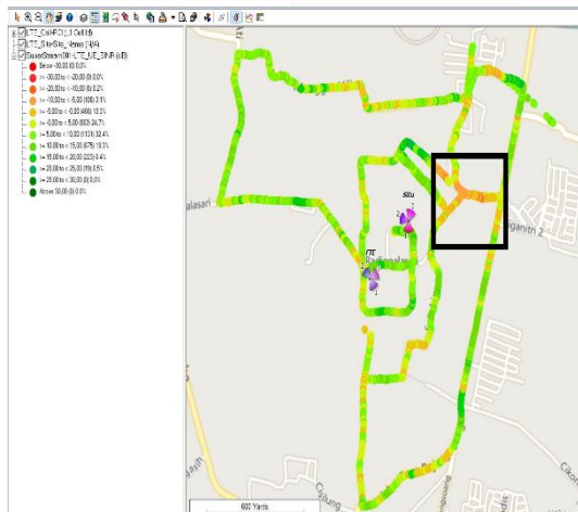
Gambar 3. Logfile SINR.
