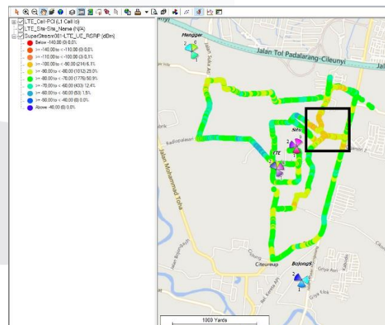
Gambar 4. Logfile RSRP.
