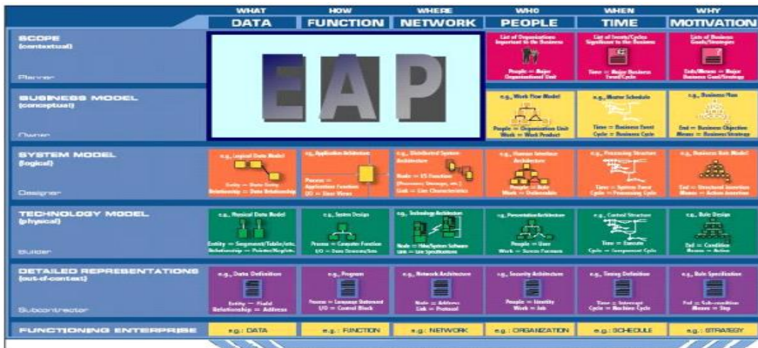
Gambar 1 matriks Zachman Framework[14]
