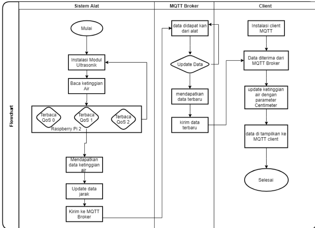
Gambar 3. Flowchart
