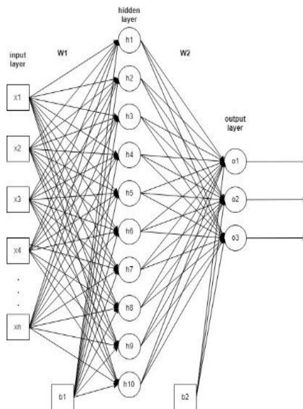
Gambar 3-2 Arsitektur Backpropagation Neural Network Multi-label
