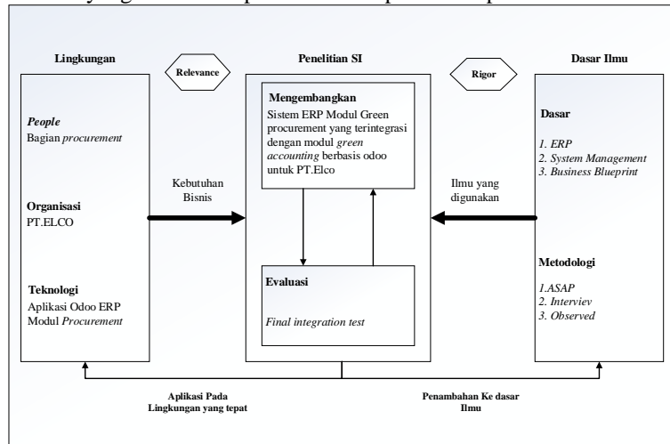
Gambar 3. 1 Konseptual Model
