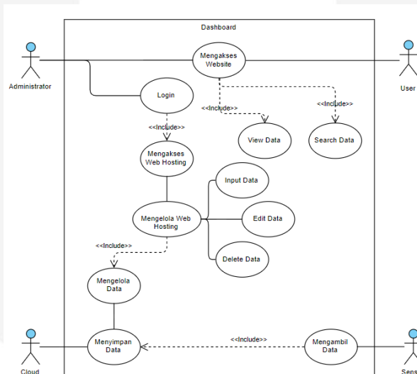
Gambar 1 Use Case Diagram Dashboard
