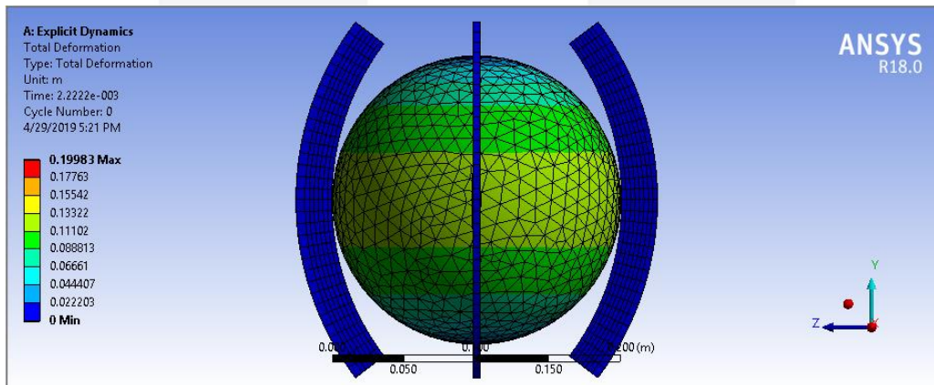
Gambar 3.5 Total Deformation
