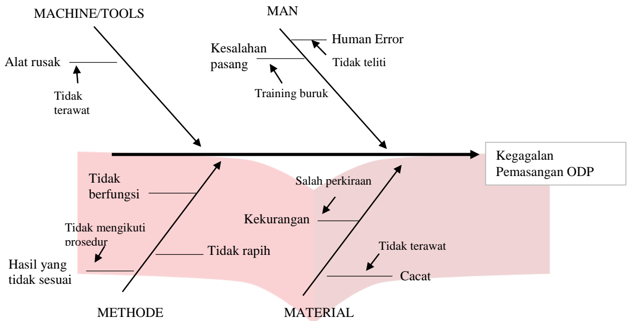
Gambar 2 Diagram Ishikawa
