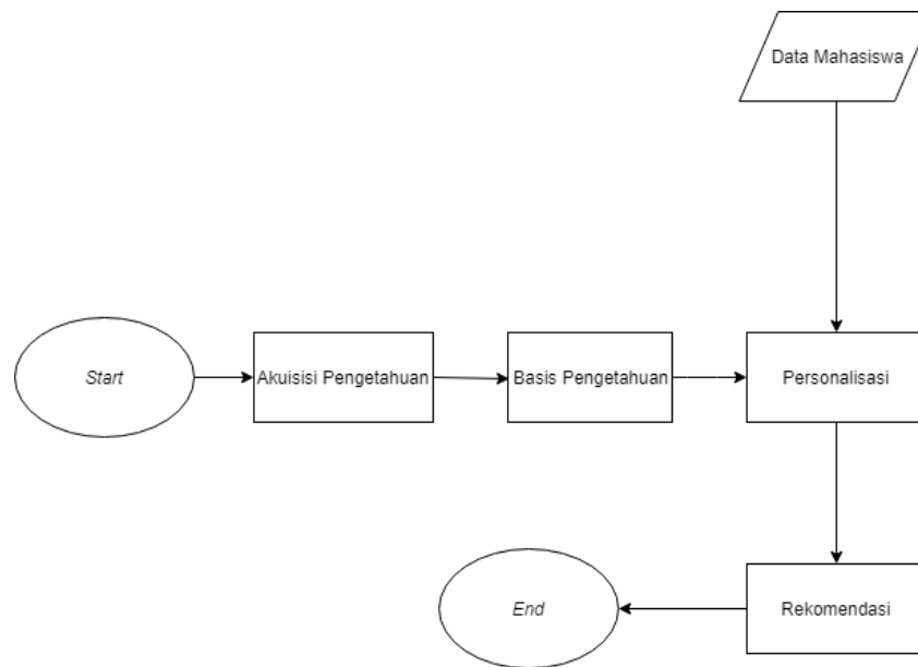
Gambar 2. Alur Penelitian
