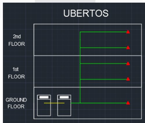
Gambar 3.7 Desain Denah Fiber to the Building Vertikal (Skenario 1)
