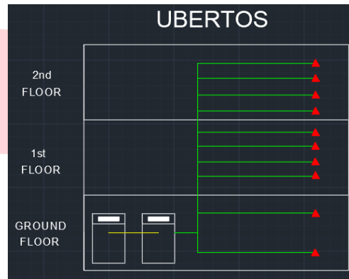
Gambar 3. 9 Desain Denah Fiber to the Building Vertikal (Skenario 3)
