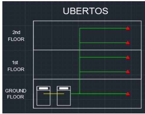
Gambar 3. 8 Desain Denah Fiber to the Building Vertikal (Skenario 2)
