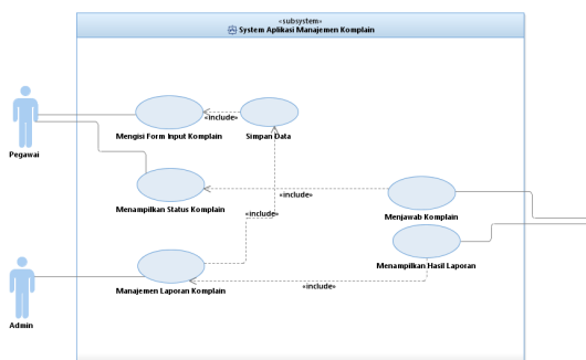
Gambar 0.1 Usecase diagram
