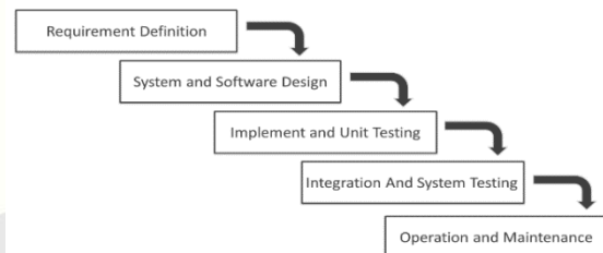
Gambar 1 - 1. Model Waterfall
