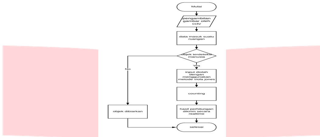
Gambar 3.3. Flowchart
