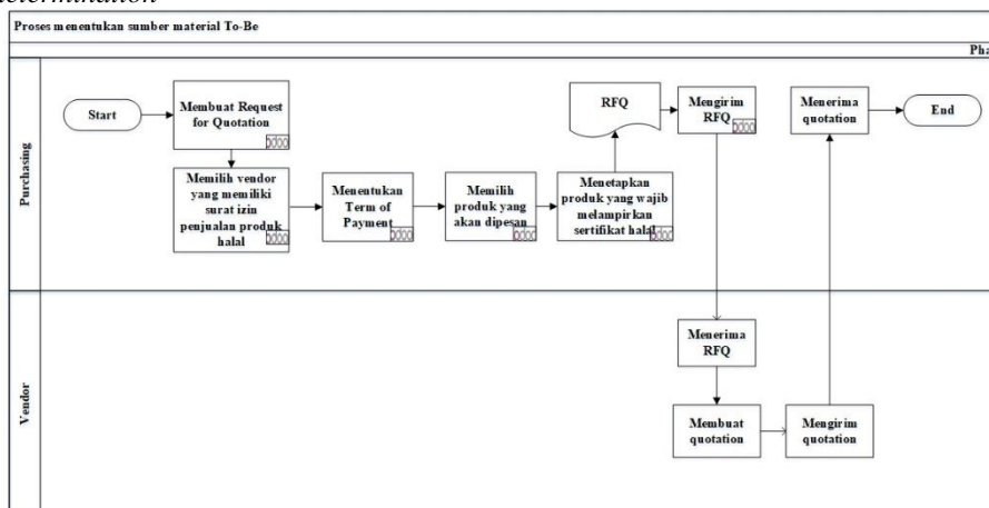
Gambar 4 Proses bisnis source determination target
