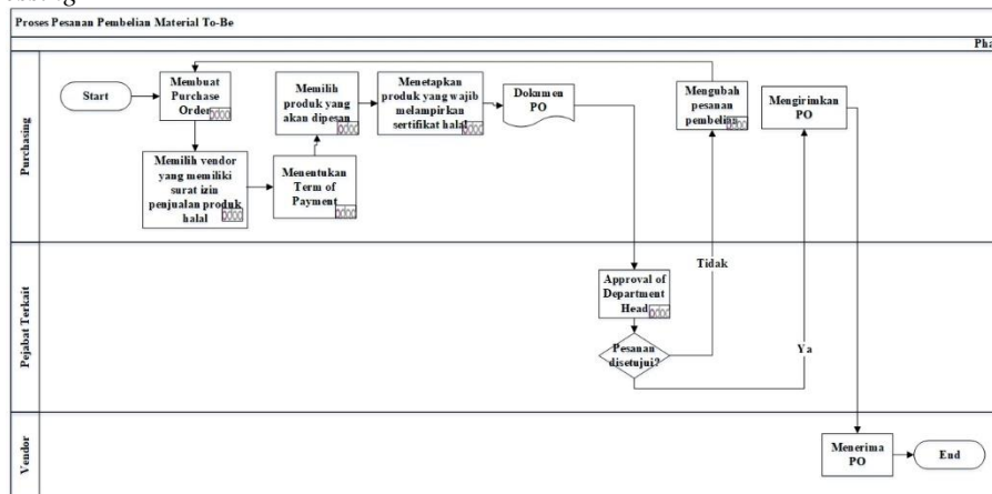
Gambar 6 Proses bisnis PO Processing target
