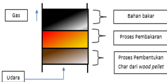
Gambar 3. Prinsip Top Lit Up Draft (T-LUD) gasifier
