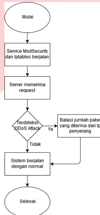
Gambar 3.4. Flowchart WAF
