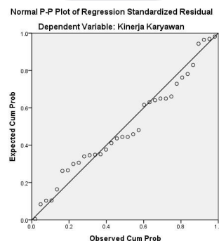
Gambar 3 Diagram P-Plot
